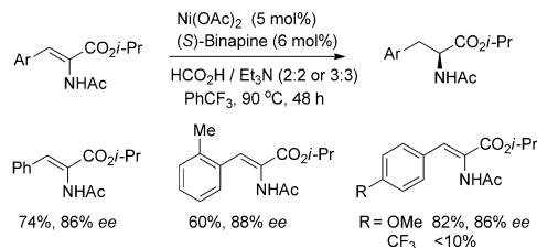
Figure 4. Asymmetric transfer hydrogenation for the synthesis of α-acetamidoesters.
